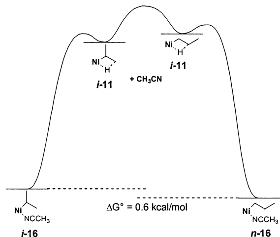
Figure 1. Free energy diagram for the isomerization of i -16 to n -16
