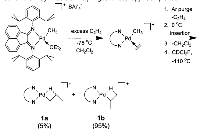
Scheme 3. Synthesis of Pd \beta -Agostic Isopropyl Complexes
