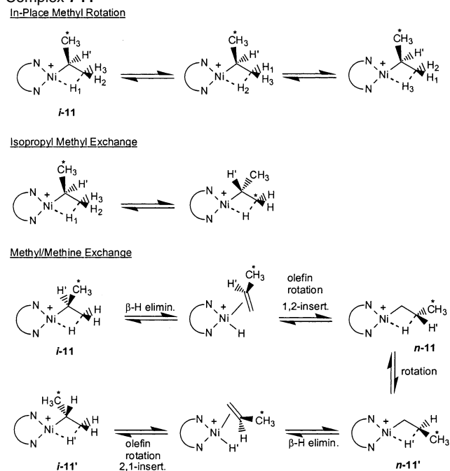
Scheme 7. Dynamic Processes Observed in \beta -Agostic Isopropyl Complex i -11
