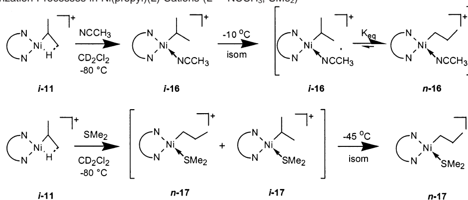
Scheme 11. Isomerization Processes in Ni(propyl)(L) Cations (L = NCCH 3 , SMe 2 )
